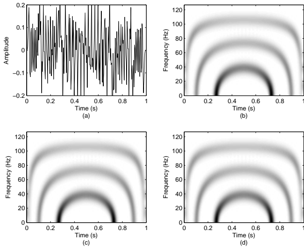
Fig. 4. The time domain representation of the consider signal is shown in (a). Spectrograms of: (b) the original signal; (c) the signal based on equal distance samples; (d) the signal based on irregular samples.
