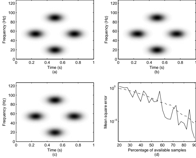
Fig. 1. Spectrograms of: (a) the original signal; (b) the signal based on uniform samples; (c) the signal based on nonuniform samples. Mean square error obtained when using various percentage of samples is shown in (d), with the solid line indicating the error obtained with uniform samples, and the dashed line indicating the error obtained with nonuniform samples.
