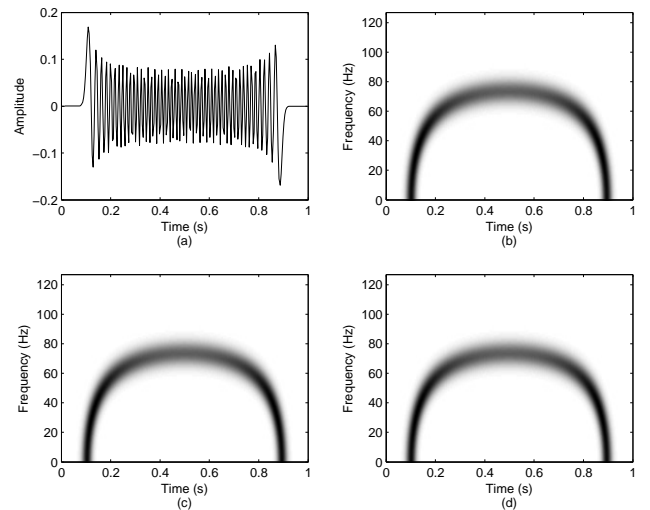
Fig. 3. The time domain representation of the consider signal is shown in (a). Spectrograms of: (b) the original signal; (c) the signal based on equal distance samples; (d) the signal based on irregular samples.
