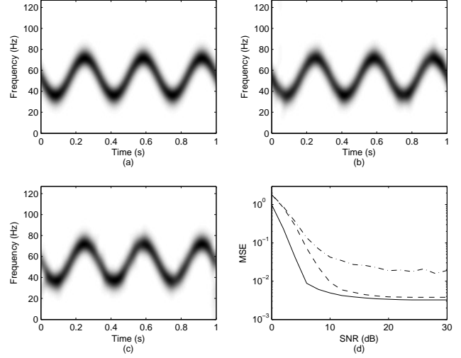
Fig. 2. Spectrograms of: (a) the original signal; (b) the signal based on equal distance samples; (c) the signal based on irregular samples. The performance of the IF estimator is shown in (d) based on the original signal (solid line), equal-distance compressed samples (dashed line) and nonuniform compressed samples (dash-dotted line).
